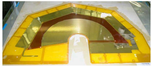
Fig. 8. The readout board glued on the support.
