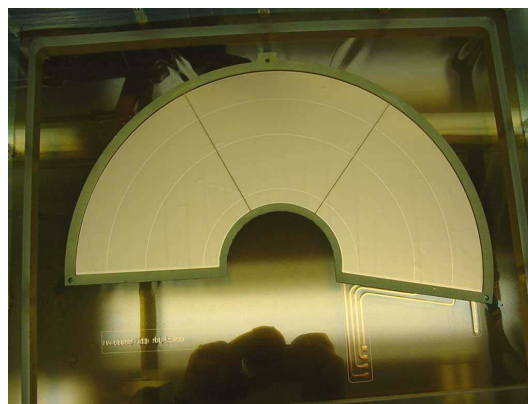
Fig. 4. The GEM foil glued on the frame.
